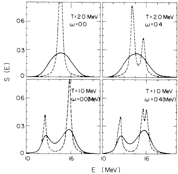
FIG. 2. Strength functions associated with the GDR in ^{166}\text{Er} as a function of the excitation energy and of the rotational frequency. The results displayed with a continuous curve were calculated making use of Eq. (6), while those displayed with a dashed curve do not contain fluctuations [Eq. (7)], and correspond to the strength functions associated with the equilibrium values (\beta_0, \gamma_0) predicted in Ref. 1. An averaging parameter \Gamma = 0.5 MeV has been used throughout.
