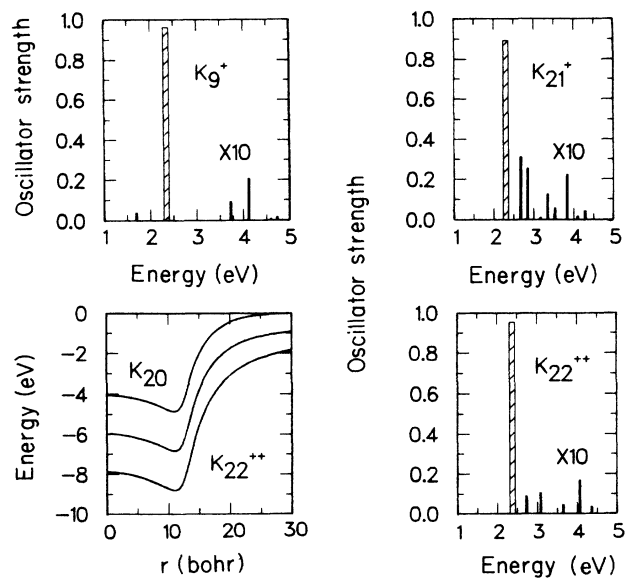
FIG. 1. Dipole oscillator strength for the charged potassium clusters K_9^+ , K_{21}^+ , and K_{22}^{2+} . Solid bars indicate values multiplied by ten. For the same number of delocalized electrons, the reduction of fragmentation with increasing positive charge is apparent. In the lower-left corner, the average potentials corresponding to K_{20} , K_{21}^+ , and K_{22}^{2+} clusters are plotted. The depth of the potentials increases by \approx 2 eV per extra charge.
