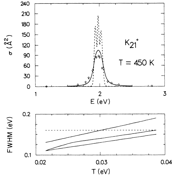
FIG. 2. Quantal size effects for K_{21}^+ : Lower part: Results for the FWHM obtained using Eqs. (1)–(4), and taking for \Gamma in Eq. (1) the parametrization of Eq. (5) with \gamma=1 (lower curve), \gamma=2 (middle curve), and \gamma=3 (upper curve). The horizontal dashed line corresponds to the experimentally determined FWHM for the range of possible temperatures of the cluster (Ref. 22). Upper part: Photoabsorption cross section. The experimental data (Ref. 6) are plotted with open circles; the dashed line displays the resulting broadening due solely to thermal fluctuations (zero intrinsic width). The full drawn curve includes the relaxation process (i) (cf. text), using the parametrization in Eq. (5) with \gamma=2 . The temperature selected corresponds to the crossing point between the middle solid and the horizontal dashed curves in the lower part of this figure.
