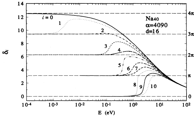
FIG. 2. Phase shifts from \ell = 0 up to \ell = 10 as a function of incident electron energy for the e^- -Na 40 system.
