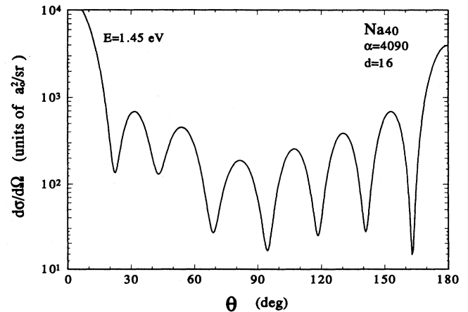
FIG. 5. Differential cross section for the system e^- -Na 40 for the incident energy E = 1.45 eV.
