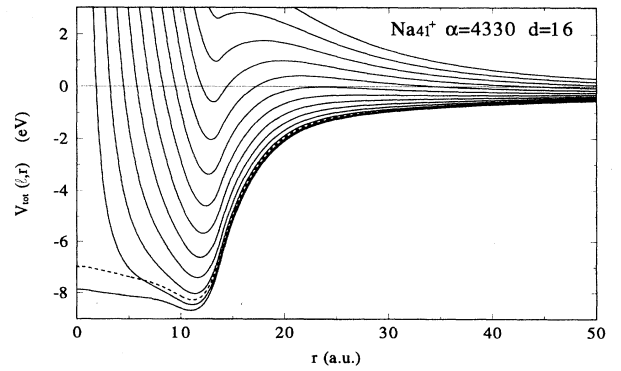
FIG. 7. Effective potentials for Na 41 + for \ell = 0 up to \ell = 12 . The contributions from the mean field, the polarization, and the centrifugal term are disentangled (solid lines). The potential without the polarization correction is shown only for \ell = 0 (dashed line).
