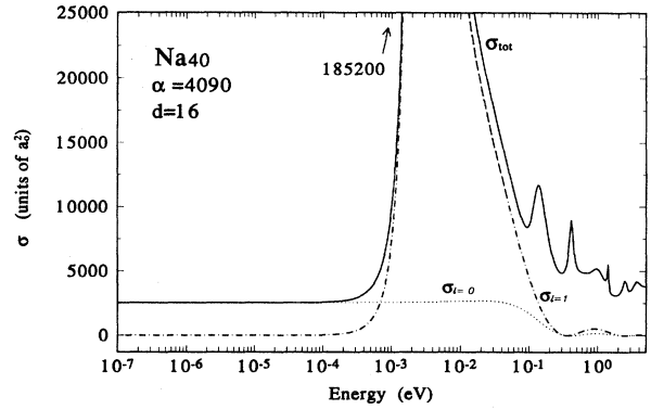
FIG. 4. Total elastic cross section for an extended range of very low incident energies for the e^- -Na 40 system. The figure shows the tendency \sigma \rightarrow \text{const} when E \rightarrow 0 .
