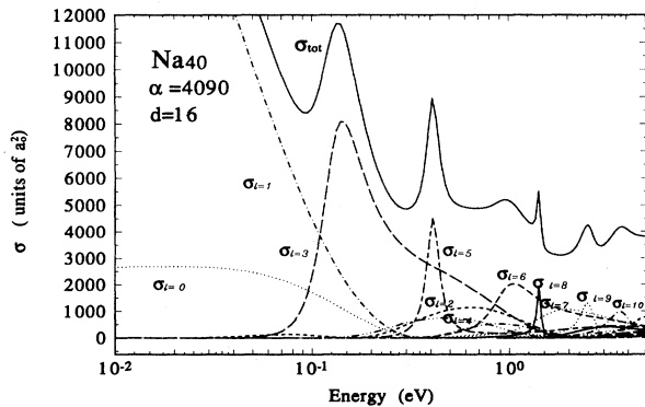
FIG. 3. Total and partial elastic cross sections as functions of the incident energy for Na 40 .
