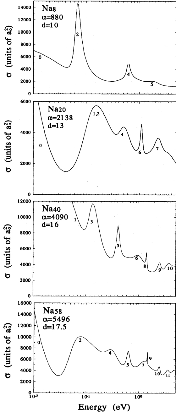
FIG. 6. Total cross sections for the systems e -Na N with N = 8, 20, 40, 58 in the same region of incoming electron energies.
