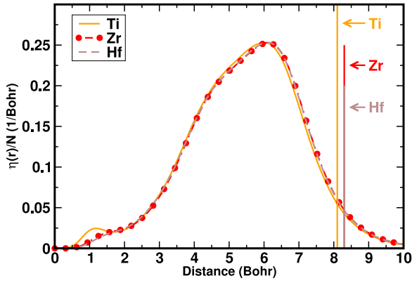
Figure 2. Normalized radial electronic densities \eta(r) = 4\pi r^2 \rho(r) plotted as a function of the distance to the central metal atom for isolated clusters \text{Ti@Si}_{16} (orange, solid line), \text{Zr@Si}_{16} (red, dash-dotted line) and \text{Hf@Si}_{16} (brown, dashed line). The radial electronic density \rho(r) is obtained from the calculated ground state total electronic density \rho(r) taking its average over the solid angle \Omega . See equation (1). The total area subtended by each curve is 1.
