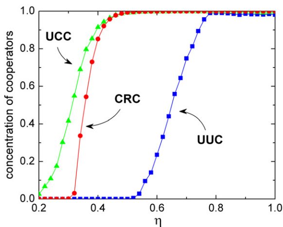
Fig. 3. Cooperation level with scale-free networks as interaction structures. The different symbols show the fraction of cooperators with different model setups as a function of the normalized multiplicative factor ( \eta ). For heterogeneous, scale-free networks, \eta is calculated using the average connectivity ( \langle k \rangle = 4 ) of the graph. Blue squares stand for the UUC cooperators, green triangles for the UCC cooperators, while red circles indicate the CRC cooperators. The definition of the strategies is given in the Methods. Scale-free networks (size of Z=1000 and average degree of \langle k \rangle = 4 ) were generated using the Barabási–Albert algorithm (Barabási and Albert, 1999). (For interpretation of the references to color in this figure legend, the reader is referred to the web version of this article.)
