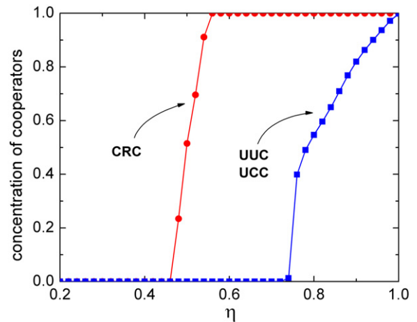
Fig. 2. Results of additional cooperator complexity on the square lattice: the fraction of cooperators as a function of the normalized multiplicative factor ( \eta ) for the different cooperator strategies. The incipient cognitive abilities of CRC cooperators make it possible to prevail under much worse conditions. Red circles show the concentration of CRC cooperators when the donations are given proportional to the payoff from the groups, while blue squares show the results of the traditional case (UUC or, equivalently, UCC), where the donations are shared equally. We used a square lattice of size Z=100 \times 100 as an example of a homogeneous interaction structure, with nearest neighbor (von Neumann) interactions ( k=4 ) and with periodic boundary conditions. (For interpretation of the references to color in this figure legend, the reader is referred to the web version of this article.)
