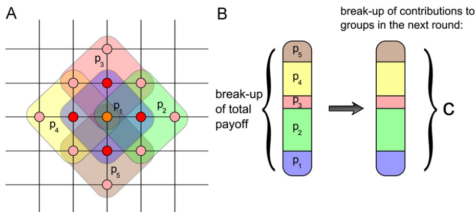
Fig. 1. Public Goods Game on graphs. (A) Players are participating in (k+1) games in every generation. Colored bubbles show the PGG groups in which the central (orange) player is participating while the p_i values show the payoff she gains from the corresponding groups. (B) Reactive behavior of CRC cooperators: colored bars show the orange player's payoff-share gained from each group (with a given color) compared to the player's total payoff. In the next generation, cooperators divide their contribution to the public good according to their previous income. (For interpretation of the references to color in this figure legend, the reader is referred to the web version of this article.)
