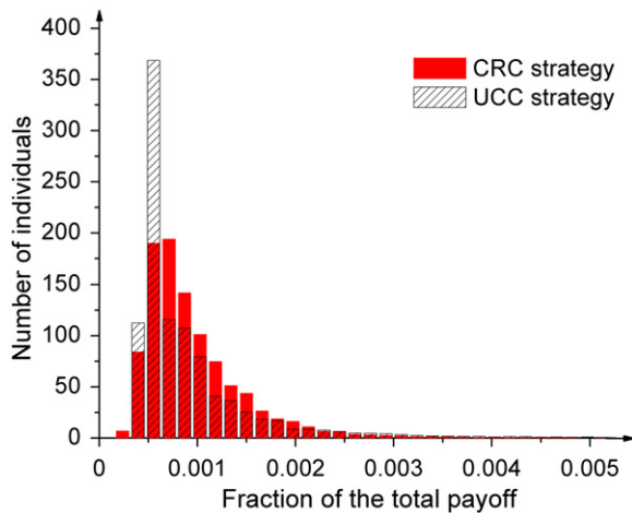
Fig. 5. Wealth distribution in fully cooperative populations for the different cooperative strategies. Red bars stand for the cognitive cooperator strategy (CRC) while striped bars show the distribution for the “equal” cooperators (UCC). CRC cooperators lead to less poor and more rich individuals. Both distributions were obtained from an average over 10 different network realizations with a size of Z=10^3 . (For interpretation of the references to color in this figure legend, the reader is referred to the web version of this article.)
