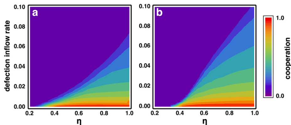
Fig. 4. Robustness against defector inflow on scale-free networks. Color codes show the cooperator concentration for different defector inflow rates as a function of \eta . After a transient period, a given amount of players were randomly replaced by defectors in every generation and the concentration values were calculated during the subsequent 10^4 generations under continuous defector inflow. The left panel (4A) displays the results for the case when cooperators share their donations equally (UCC), while the right panel (4B) shows them for the more complex, reactive cooperator strategy (CRC). CRCs are more robust against the invasion of a minority of free-riders, specially for large \eta and defectors inflow rates. (For interpretation of the references to color in this figure legend, the reader is referred to the web version of this article.)
