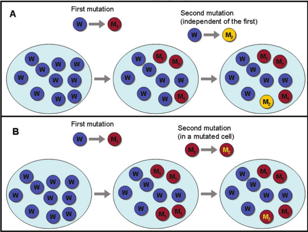
Fig. 11.3 Multiple mutations in cell populations. The probability that mutated cells acquire additional mutations depends on the number of cells at risk, which in turns depends on the fitness of the original mutant clone. The mathematical model allows us to infer that, whenever we find two different mutations, the
